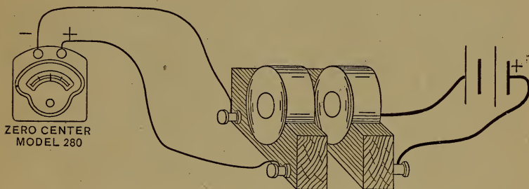
FIG. 9.—CURRENT INDUCED BY ELECTROMAGNETISM. Turner's Method.
